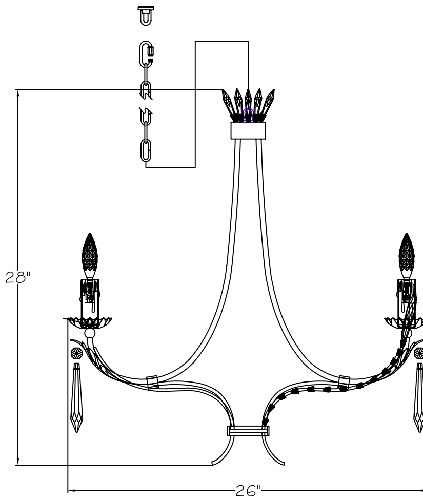
FRONT VIEW
